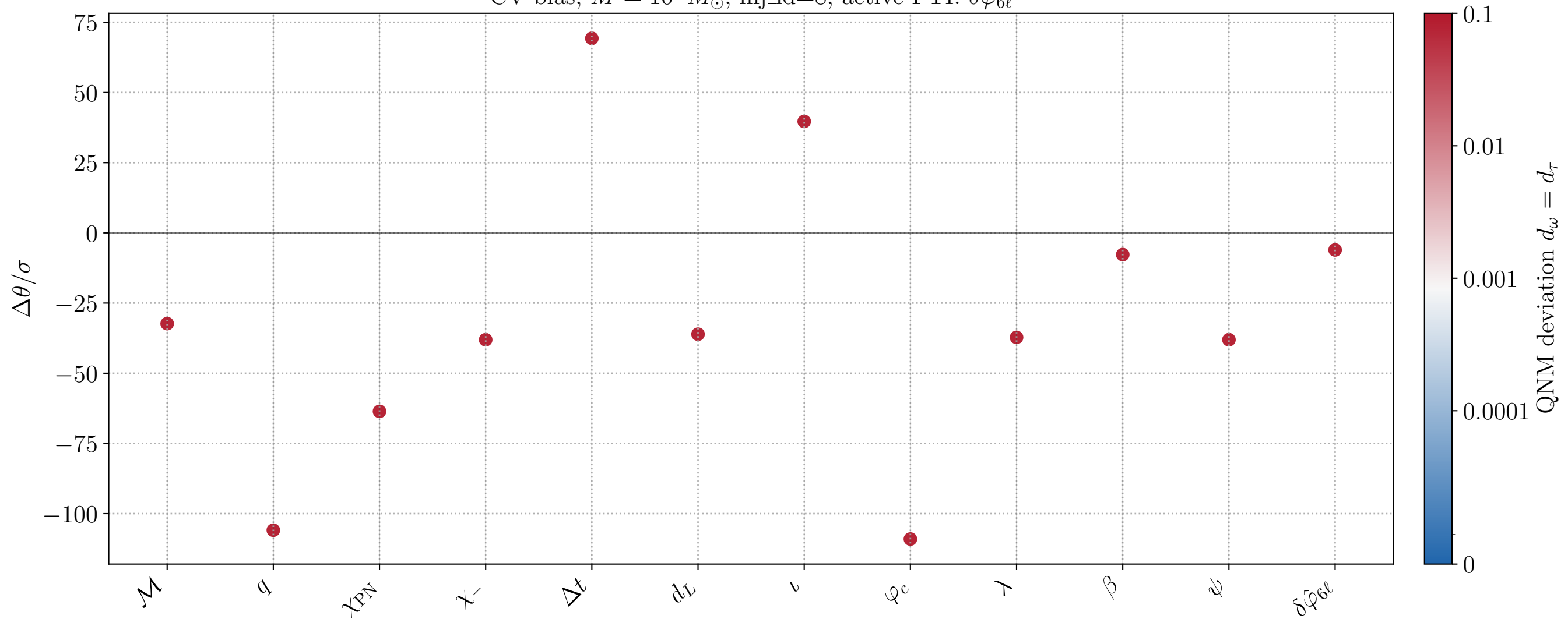
CV bias, M = 10^6 M_\odot , inj_id=8, active FTI: \delta\hat{\varphi}_{6\ell}
