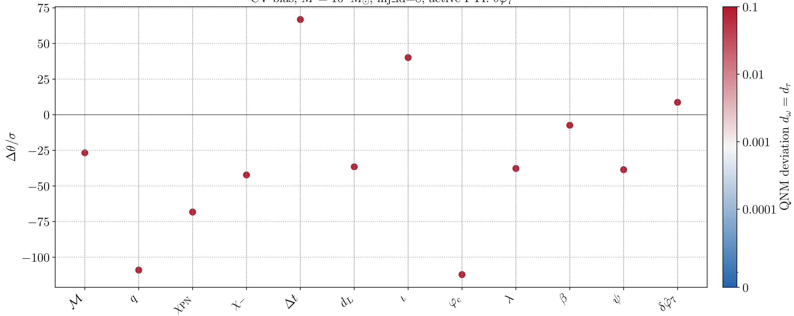
CV bias, M = 10^6 M_\odot , inj_id=8, active FTL: \delta\hat{\varphi}_7
