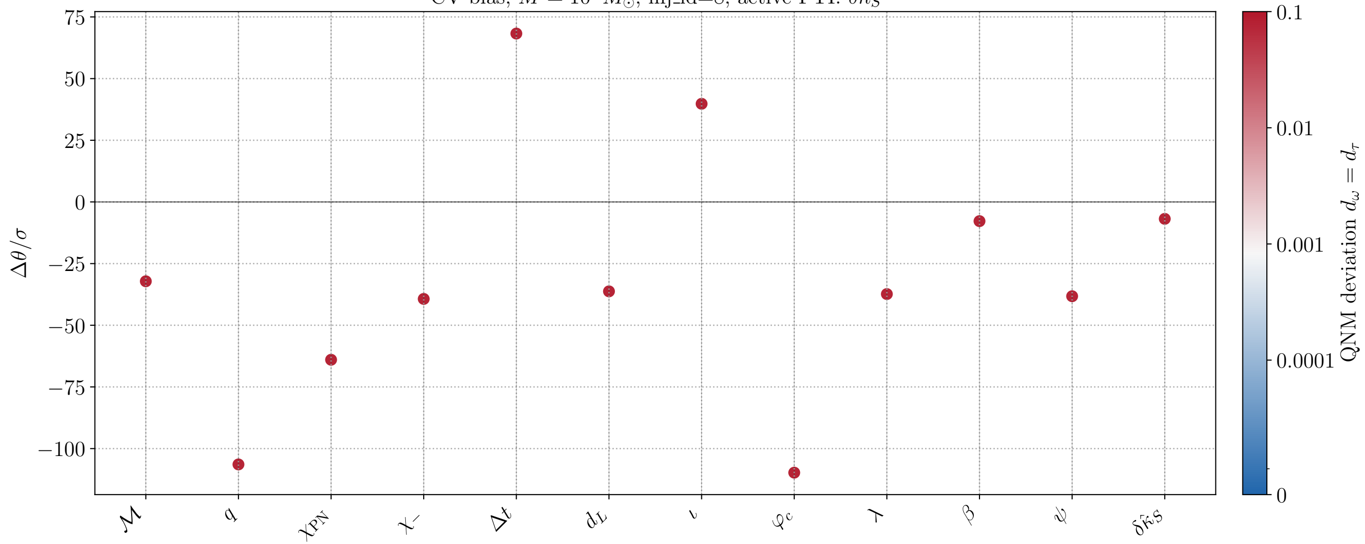
CV bias, M = 10^6 M_\odot , inj_id=8, active FTL: \delta\hat{\kappa}_S
