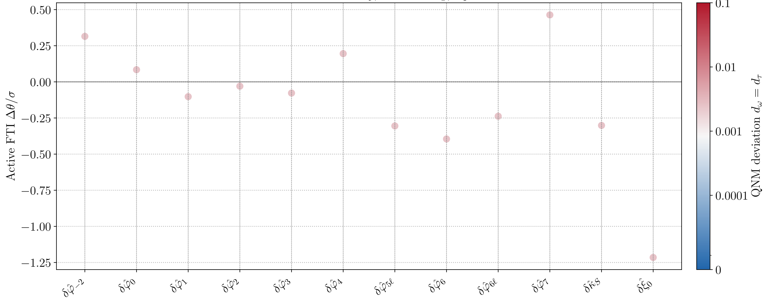
Active-FTI bias summary, M = 10^6 M_\odot , inj_id=9
