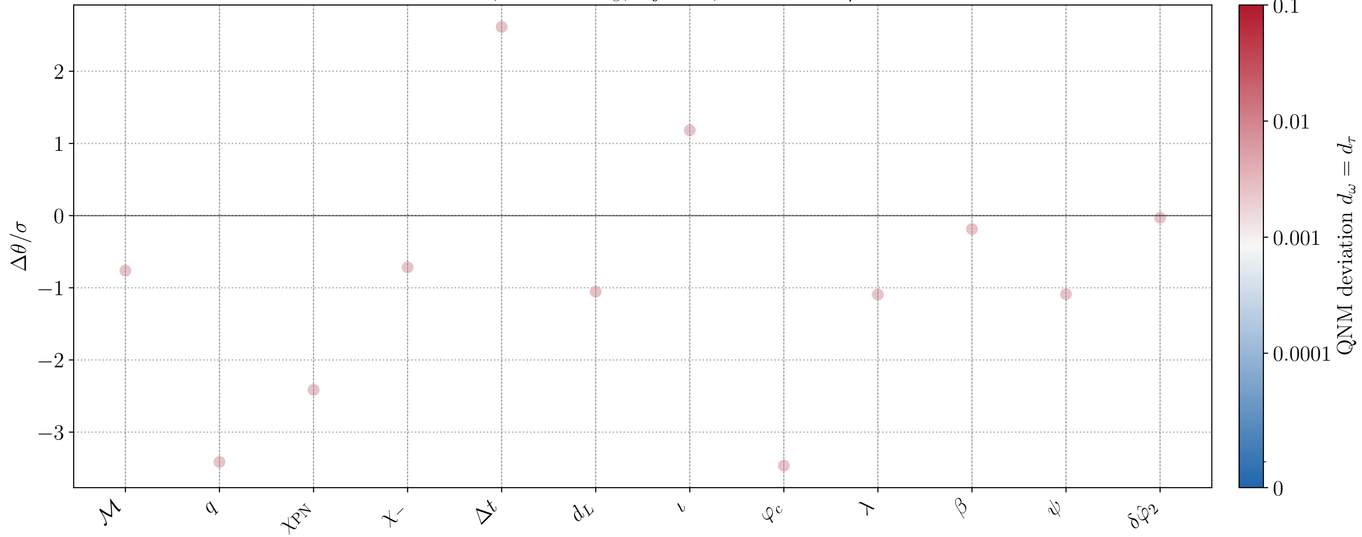
CV bias, M = 10^6 M_\odot , inj_id=9, active FTI: \delta\hat{\varphi}_2
