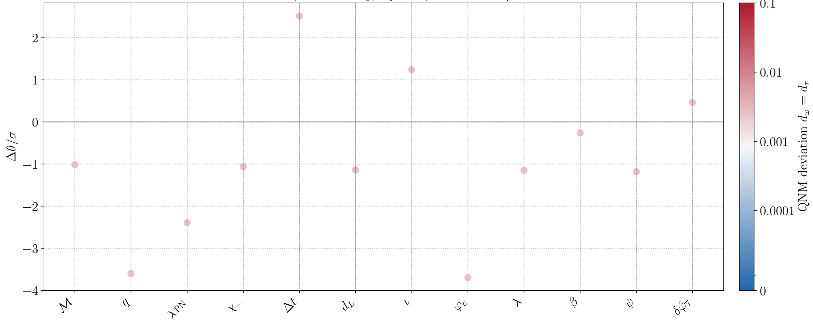
CV bias, M = 10^6 M_\odot , inj_id=9, active FTI: \delta\hat{\varphi}_7
