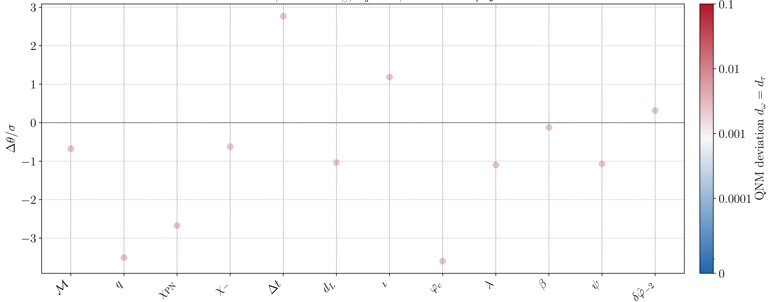
CV bias, M = 10^6 M_\odot , inj_id=9, active FTL: \delta\hat{\varphi}_{-2}
