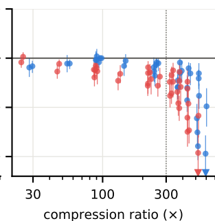
Watershed (12 frames)
