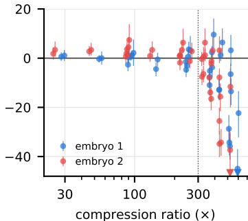
LoG (12 frames)
