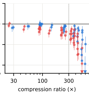
Watershed (12 frames)
