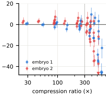
LoG (12 frames)
