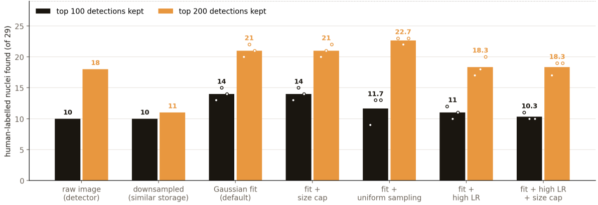
Figure 6: Human-labelled nuclei found in the top 100 and top 200 detections per method (bars: mean; dots: seeds). The LoG baseline of Table 7 is not drawn: it exceeds every fit in the top 100 (16–18), and in the top 200 (22) it is level with the uniform-sampling fit (22.7).
