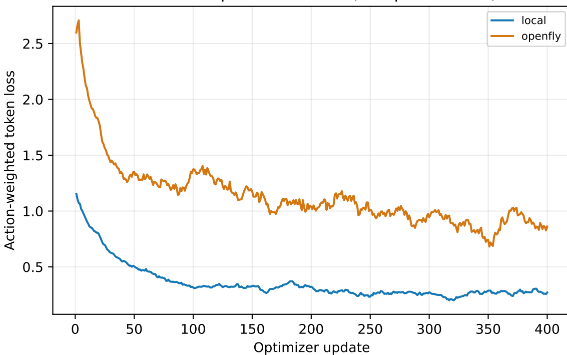
qwen / optimization loss (20-update mean)
