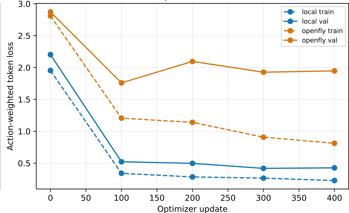
smol500 / fixed-probe evaluation-mode loss
