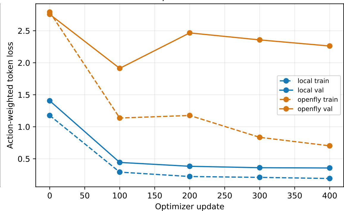
qwen / fixed-probe evaluation-mode loss
