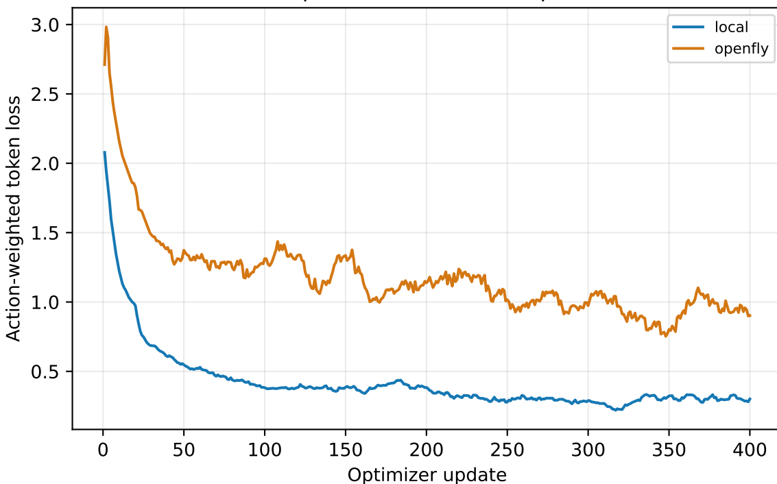
smol500 / optimization loss (20-update mean)
