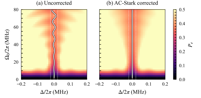
Figure 4. Echo-root-Lorentzian spectroscopy without (a) and with (b) accumulated-phase compensation of drive-induced center motion. The maps show the measured excited-state population for L = 20 \mu s, cutoff c = 0.001 , and \beta = 0 ; the applied correction is \kappa = 0.00225 \text{ MHz}^{-1} . White curves mark the fitted spectral centers. The dashed line marks zero detuning, and the paired dotted lines at \Delta/(2\pi) = \pm\Gamma_{f,T_2}/2 enclose the coherence-limited FWHM \Gamma_{f,T_2} = 1/(\pi T_{2,\text{eff}}) = 43.5 \text{ kHz} . The common color scale is clipped at P_e = 0.5 for visibility. The uncorrected center oscillates with drive amplitude, whereas the corrected center remains pinned near zero detuning.
