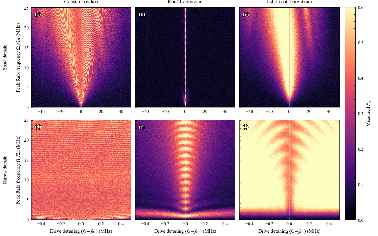
Figure 2. Experimental q1 spectroscopy maps for 20 \mu\text{s} pulses. The color scale is the state-discriminated, measured excited-state population P_e . The upper row shows the broad 100 MHz domain ( -50 to +50 MHz) with 0.5 MHz spacing; the lower row shows the narrow 1 MHz domain ( -0.5 to +0.5 MHz) with 5 kHz spacing. From left to right, the columns show a nearly constant-envelope echo implemented as a root-Lorentzian with a midpoint phase inversion, an ordinary root-Lorentzian with c = 0.005 , and an echo-root-Lorentzian with c = 0.005 . All broad maps and the narrow constant-envelope map contain 200 shots per point. The narrow ordinary-pulse run contains 216 completed averages per point despite requesting 1000, while the narrow echo-root-Lorentzian run contains all 1000. All panels use the same 200-point calibrated peak-Rabi grid, extending from zero to approximately 25.1 MHz, and the same probability scale. Active reset and state-discriminated readout are used throughout. The white dashed line denotes the programmed zero detuning.
