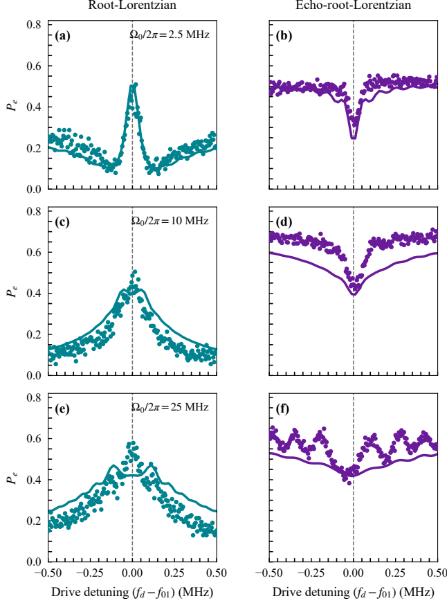
Figure 3. Experimental and simulated spectra. (a)–(f) Final excited-state probability P_e versus detuning for 20 \mu s root-Lorentzian (left) and echo-root-Lorentzian (right) pulses with c = 0.005 . From top to bottom, \Omega_0/2\pi = 2.5, 10 , and 25 MHz. Colored continuous lines show three-level simulations evaluated with 3000 temporal grid points, and colored markers show the 10 August 2026 q1 OPX1000 data.
