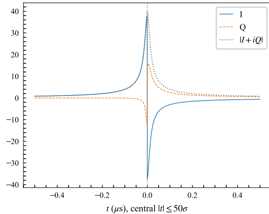
Accumulated-phase pulse
