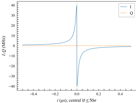
Original pulse
