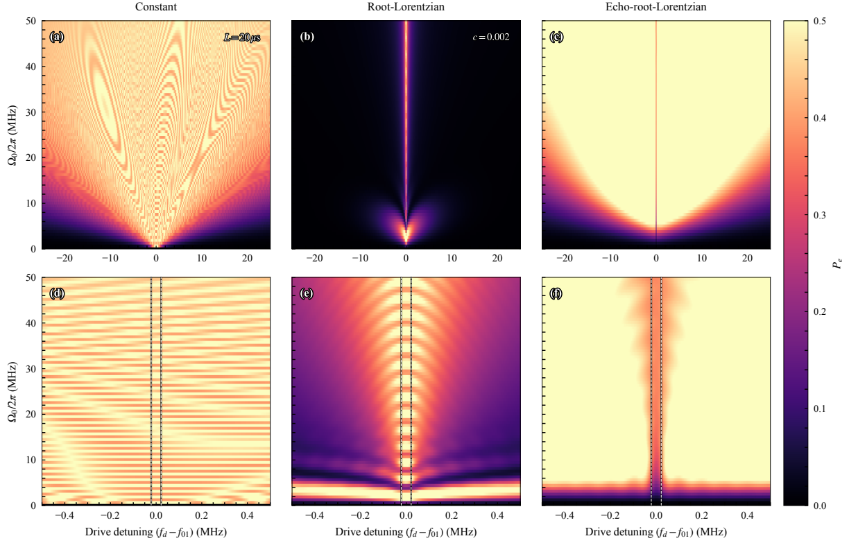
Figure 2. Experimental spectroscopy maps at two frequency scales for 20 \mu\text{s} pulses. The color scale is the measured excited-state population P_e . The upper row shows the broad 50 MHz domain ( -25 to +25 MHz), and the lower row shows the narrow 1 MHz domain ( -0.5 to +0.5 MHz). In the narrow panels, the paired black-edged white dashed lines at \Delta/(2\pi) = \pm\Gamma_{f,T_2}/2 enclose the coherence-limited FWHM; no reference line is drawn in the broad panels. From left to right, the columns show the constant, root-Lorentzian, and echo-root-Lorentzian protocols; the shaped pulses use relative endpoint amplitude c = 0.002 . All six panels use the same peak-Rabi grid and probability scale. The comparison exposes conventional power broadening for the constant pulse, amplitude-dependent coherent structure for the ordinary root-Lorentzian pulse, and the narrow resonance-centered depletion feature preserved by the echo phase inversion.
