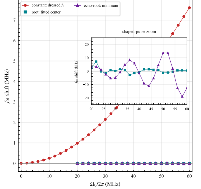
Figure 4. Drive-induced f_{01} displacement in the three-level model over an extended peak-Rabi-frequency range. The curves show the exact constant-pulse dressed shift, the fitted center of the root-Lorentzian central spectral envelope, and the echo-root-Lorentzian central minimum. The inset expands the shaped-pulse shifts to \pm 25 kHz. The finite shaped-pulse positions include coherent interference and are operational spectral centers rather than instantaneous dressed-state shifts.
