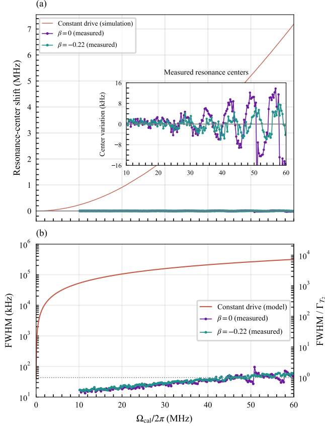
Figure 5. Resonance-center stability and linewidth of the measured echo-root-Lorentzian response. (a) Measured center variations compared with the simulated constant-drive AC-Stark shift. The measured curves use the same fitted centers as Fig. 4 for \beta = 0 and -0.22 . The inset resolves their amplitude-dependent fluctuations over 10–60 MHz: the \beta = -0.22 waveform exhibits smaller center variations. The constant-drive curve retains the three-level simulation with \alpha/(2\pi) = -216.0 MHz. (b) Gaussian-fit FWHM of the same measured spectra and the red constant-drive power-broadening reference, on a logarithmic scale. The right axis expresses linewidths in units of the paper’s q1 reference \Gamma_{T_2} = 43.5 kHz (dotted line). Both measured waveforms broaden with drive, while the \beta = 0 response exhibits larger linewidth excursions at high amplitudes.
