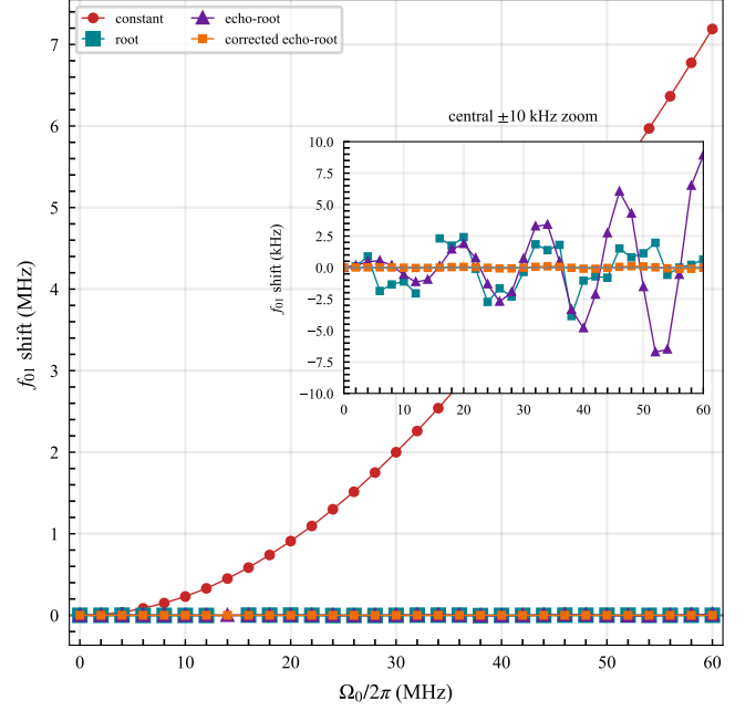
Figure 5. Measured drive-induced f_{01} displacement over an extended peak-Rabi-frequency range. The curves connect the measured spectral centers for the constant-pulse and root-Lorentzian references and for the uncorrected and accumulated-phase-corrected echo-root-Lorentzian response. The root reference uses L = 10 \mu\text{s} and c = 0.002 ; both echo curves use L = 20 \mu\text{s} , c = 0.001 , \beta = 0 , and \alpha/(2\pi) = -216.0 \text{ MHz} , with \kappa = 0.00225 \text{ MHz}^{-1} for the corrected curve. The inset shows a \pm 10 \text{ kHz} center-frequency zoom; uncorrected echo points outside that window are clipped. These finite-pulse positions are operational spectral centers rather than instantaneous dressed-state shifts.
