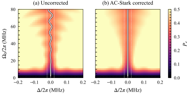
Figure 4. Echo-root-Lorentzian spectroscopy without (a) and with (b) accumulated-phase compensation of drive-induced center motion. The maps show the measured excited-state population for L = 20 \mu\text{s} , cutoff c = 0.001 , and \beta = 0 ; the applied correction is \kappa = 0.00225 \text{ MHz}^{-1} . White curves mark the fitted spectral centers. The dashed line marks zero detuning, and the paired dotted lines at \Delta/(2\pi) = \pm\Gamma_{f,T_2}/2 enclose the coherence-limited FWHM \Gamma_{f,T_2} = 1/(\pi T_{2,\text{eff}}) = 43.5 \text{ kHz} . The common color scale is clipped at P_e = 0.5 for visibility. The uncorrected center oscillates with drive amplitude, whereas the corrected center remains pinned near zero detuning.
