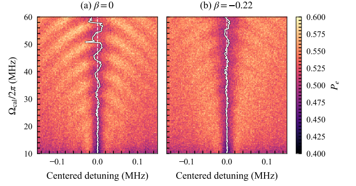
Figure 4. Measured q6 echo-root-Lorentzian spectroscopy for (a) \beta = 0 and (b) \beta = -0.22 , with L = 50 \mu\text{s} and cutoff c = 0.00075 . White curves trace the fitted resonance centers. Over the 10–60 MHz drive range, the \beta = -0.22 waveform shows smaller amplitude-dependent fluctuations of the resonance center, while preserving the narrow depletion feature. This waveform combines a DRAG quadrature with a smoothed midpoint inversion.
