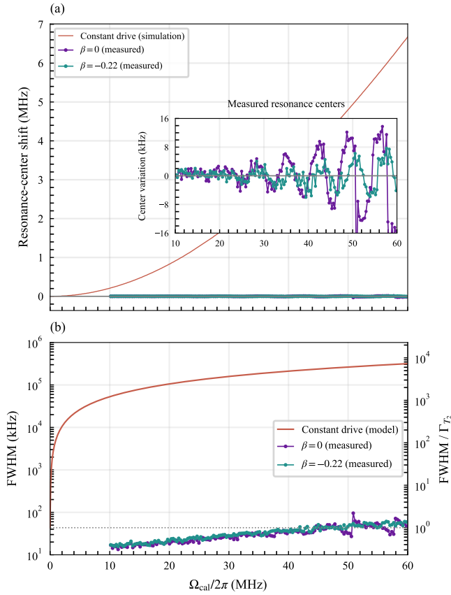
Figure 5. Resonance-center stability and linewidth of the measured echo-root-Lorentzian response. (a) Measured center variations compared with the simulated constant-drive AC-Stark shift. The measured curves use the same fitted centers as Fig. 4 for \beta = 0 and -0.22 . The inset resolves their amplitude-dependent fluctuations over 10–60 MHz: the \beta = -0.22 waveform exhibits smaller center variations. The constant-drive curve uses the q6 anharmonicity in the three-level simulation. (b) Gaussian-fit FWHM of the same measured spectra and the red constant-drive power-broadening reference, on a logarithmic scale. The right axis expresses linewidths in units of the paper’s q1 reference \Gamma_{T_2} = 43.5 kHz (dotted line). Both measured waveforms broaden with drive, while the \beta = 0 response exhibits larger linewidth excursions at high amplitudes.
