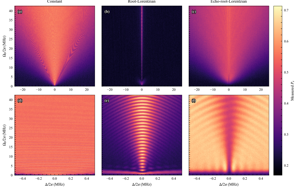
Figure 2. Experimental q1 spectroscopy maps for 20 \mu\text{s} pulses. From left to right: constant, root-Lorentzian, and echo-root-Lorentzian pulses, with c = 0.005 for both shaped pulses. The Lorentzian pulses produce extremely narrow resonance features compared with the power-broadened constant-pulse response. The ordinary root-Lorentzian response retains pronounced coherent oscillations as the drive amplitude increases. The echo suppresses these oscillations, revealing a narrow, persistent resonance-centered depletion feature across the measured drive range.
