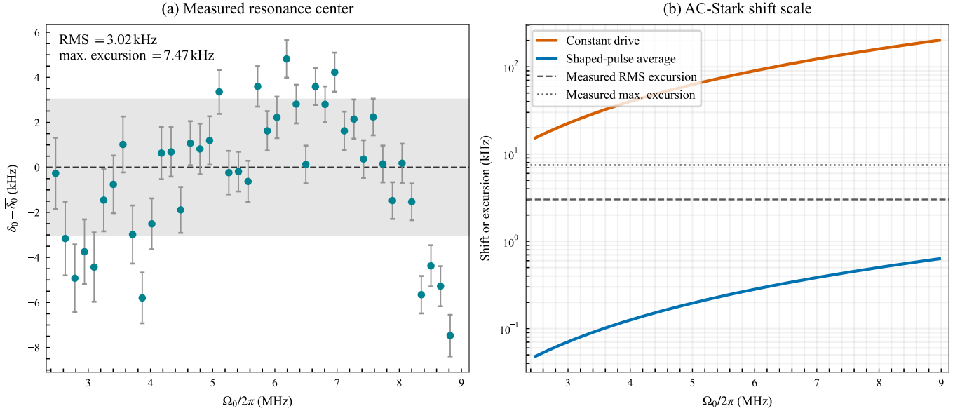
Figure 4. Direct test of resonance-center robustness against drive amplitude. (a) Measured q1 center displacement relative to the inverse-variance weighted mean over the independently selected Q \geq 0.10 operating window. Vertical bars are one-standard-deviation covariance uncertainties, the dashed line is the weighted mean, and the gray band spans the empirical RMS displacement of \pm 3.02 kHz. The maximum absolute displacement is 7.47 kHz; no center-position gate is used. (b) Weak-drive AC-Stark scales over the same amplitude interval. The constant-drive curve uses the three-level transmon estimate with \alpha/(2\pi) = -200 MHz; the shaped-pulse curve includes the root-Lorentzian phase-average factor \langle f^2 \rangle_t = 0.003138 . Horizontal lines mark the measured RMS and maximum excursions. The shaped pulse strongly separates peak drive amplitude from the expected Stark displacement, consistent with the absence of a monotonic quadratic shift in panel (a).
