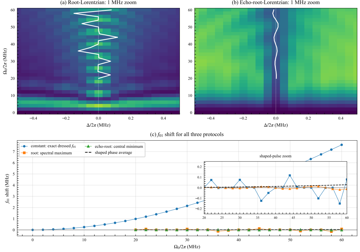
Figure S17. Fine f_{01} comparison for the Lorentzian-derived pulses and all three resonance shifts. (a),(b) One-megahertz central zooms of the root-Lorentzian and echo-root-Lorentzian final excitation, respectively. The dotted line marks the bare f_{01} frequency and the solid lines mark the extracted maximum or central minimum. (c) Constant-pulse exact dressed shift, root-Lorentzian maximum, echo-root-Lorentzian central minimum, and the common shaped-pulse phase-average estimate. The inset expands the shaped-pulse shifts to \pm 0.25 MHz.
