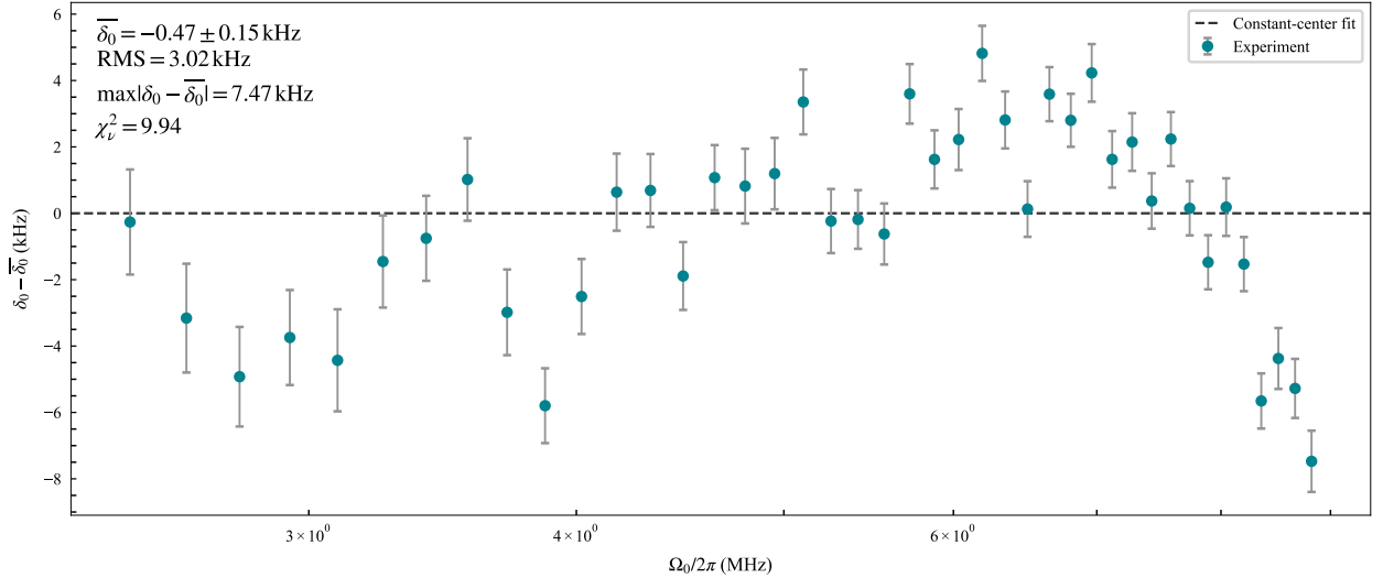
Figure S11. Direct amplitude-robustness test from the fitted resonance center. Markers show \delta_0(\Omega_0) - \overline{\delta_0} for the 42 measured slices in the independently selected Q \geq 0.10 operating window; vertical bars are one-standard-deviation center uncertainties from the Gaussian-fit covariance. The dashed zero line is the inverse-variance-weighted constant-center fit. Center itself is not used as a quality gate for this panel. The residual RMS is 3.02 kHz and the maximum absolute deviation is 7.47 kHz; reduced \chi^2 = 9.94 shows that the small residual structure is nevertheless resolved relative to the local fit uncertainties.
