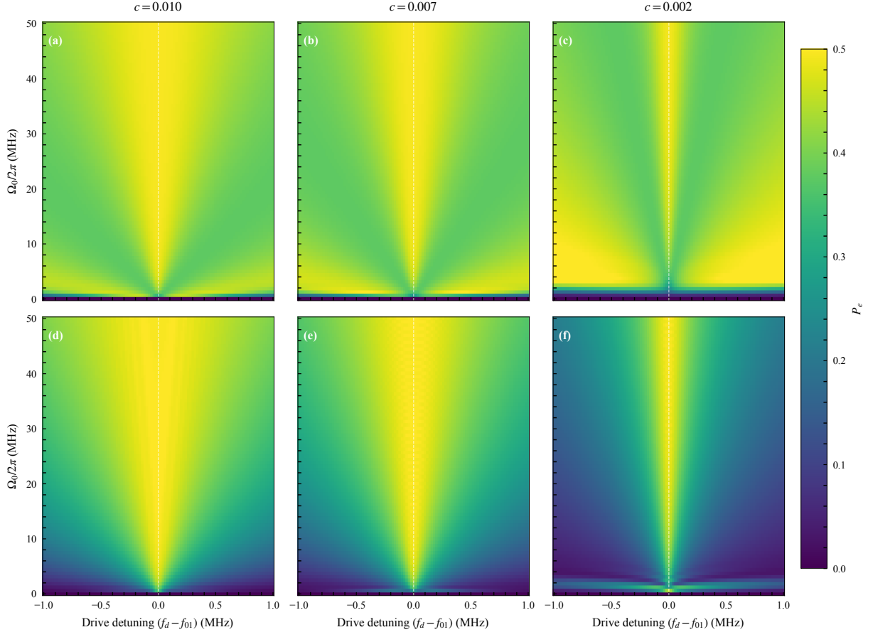
Figure S16. Simulated cutoff comparison for L = 60 \mu\text{s} , using the same layout, axes, color scale, and model parameters as Fig. S14.
