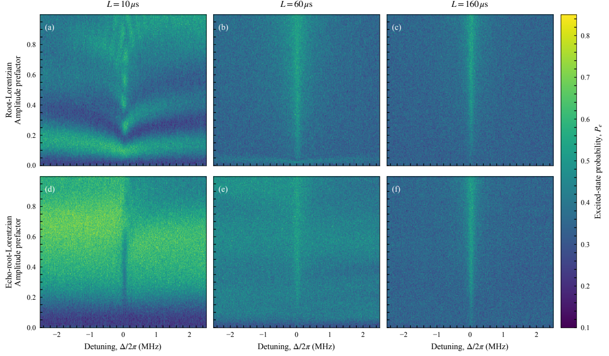
Figure S12. Experimental pulse-duration comparison on qubit q9. The top row shows root-Lorentzian spectroscopy and the bottom row shows the matched echo-root-Lorentzian protocol for L = 10, 60 , and 160 \mu\text{s} . Each panel reports the measured excited-state probability over the same detuning and amplitude-prefactor grid; all panels share one color scale. The short root-Lorentzian scan exhibits pronounced amplitude-dependent structure, whereas the echo data are smoother. By L = 160 \mu\text{s} , both protocols have converged toward essentially the same response: a narrow resonance-centered line on a common relaxation-dominated background.
