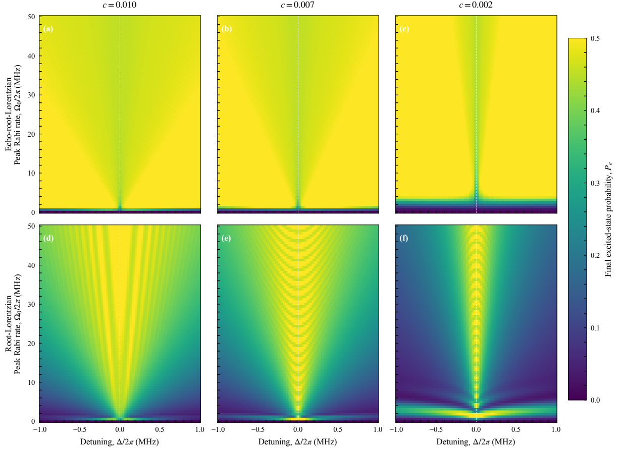
Figure S15. Simulated cutoff comparison for L = 30 \mu\text{s} , using the same layout, axes, color scale, and model parameters as Fig. S13.
