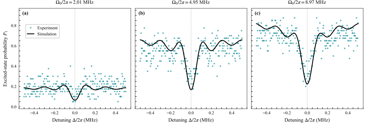
Figure S9. Measured (colored markers) and simulated (black curves) fixed-amplitude spectra at calibrated peak Rabi frequencies \Omega_0/2\pi = 2.011 , 4.951 , and 8.973 MHz. The vertical dotted line denotes zero detuning. For visual clarity, every fourth measured detuning point is displayed; all 1001 points enter the linewidth analysis. The simulation uses the parameters of Fig. S8 without a readout rescaling or fitted frequency shift.
