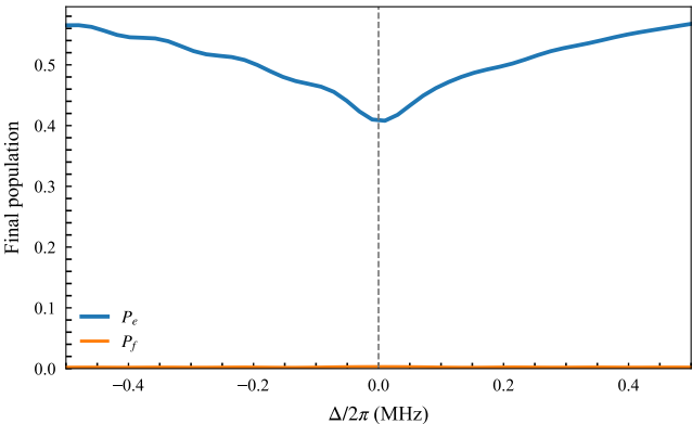
Echo-root-Lorentzian, \Omega_0/2\pi = 15 MHz
