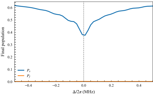
Echo-root-Lorentzian, \Omega_0/2\pi = 15 MHz, c = 0.0025
