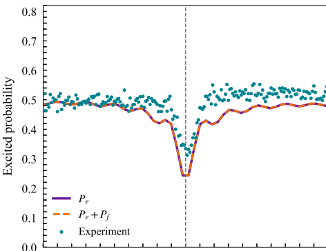
Echo-root-Lorentzian: 3-level sim. L = 20\mu\text{s} , c = 0.005 ; experiment L = 20\mu\text{s} , c = 0.005
