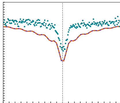
Echo-root-Lorentzian: 3-level sim. L = 20\mu\text{s} , c = 0.005 ; experiment L = 20\mu\text{s} , c = 0.005
