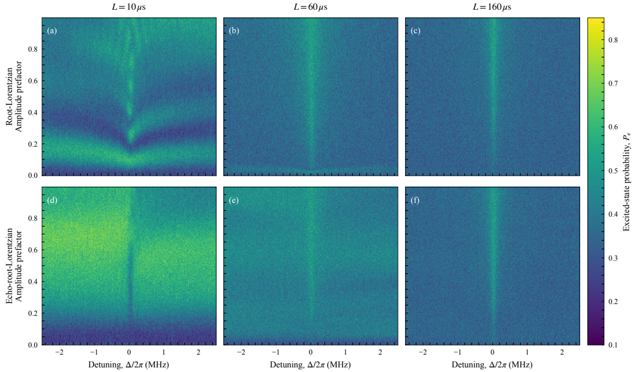
Figure S6. Experimental pulse-duration comparison on qubit q9. The top row shows root-Lorentzian spectroscopy and the bottom row shows the matched echo-root-Lorentzian protocol for L = 10, 60 , and 160 \mu\text{s} . Each panel reports the measured excited-state probability over the same detuning and amplitude-prefactor grid; all panels share one color scale. The short root-Lorentzian scan exhibits pronounced amplitude-dependent structure, whereas the echo data are smoother. By L = 160 \mu\text{s} , both protocols have converged toward essentially the same response: a narrow resonance-centered line on a common relaxation-dominated background.
