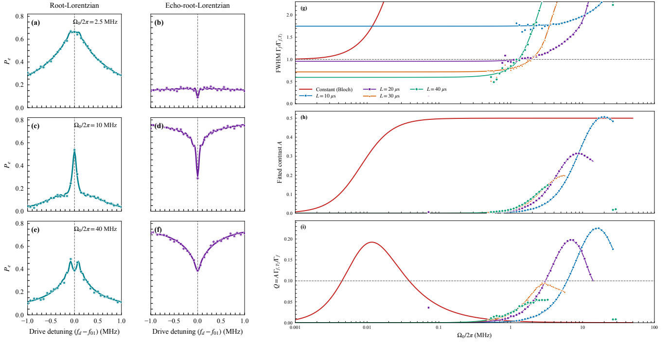
Figure 3. Spectra and resolution-contrast performance. (a)–(f) Final excited-state probability P_e versus detuning for 20\ \mu\text{s} root-Lorentzian (left) and echo-root-Lorentzian (right) pulses with c = 0.002 . From top to bottom, \Omega_0/2\pi = 2.5, 10 , and 40\ \text{MHz} . Solid curves are simulations, and markers are experimental data. Panels (g)–(i) show metrics versus peak Rabi frequency up to 50\ \text{MHz} for echo-root-Lorentzian pulses with L = 10, 20, 30 , and 40\ \mu\text{s} . Colored continuous lines show simulations, and colored markers show experimental data. (g) Fitted FWHM in units of the coherence-limited reference, \Gamma_f/\Gamma_{f,T_2} , with the dashed line marking \Gamma_f/\Gamma_{f,T_2} = 1 ; (h) fitted contrast A ; and (i) contrast-weighted resolution Q = AR = A\Gamma_{f,T_2}/\Gamma_f . The red curve is the constant-drive Bloch result, and the dashed line in (i) marks Q = 0.10 .
