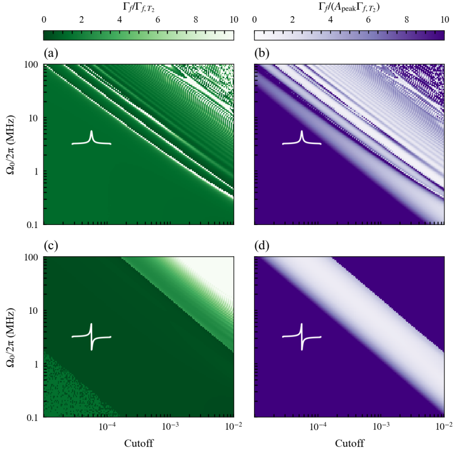
Figure S4. Numerical cutoff–amplitude maps for root-Lorentzian L^{(1/2)} and echo-root-Lorentzian L_{\text{echo}}^{(1/2)} pulses of duration 50 \mu\text{s} . (a,c) Normalized cyclic-frequency FWHM \Gamma_f/\Gamma_{f,T_2} for the root and echo protocols, respectively; (b,d) corresponding contrast-weighted widths \Gamma_f/(A_{\text{peak}}\Gamma_{f,T_2}) . The ordinary root-Lorentzian response is strongly oscillatory, whereas the echo variant retains a broader contiguous region with a favorable resolution–signal trade-off.
