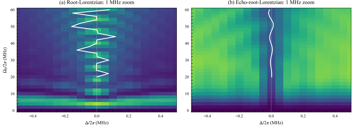
Figure S13. Fine f_{01} comparison for the Lorentzian-derived pulses. (a),(b) One-megahertz central zooms of the root-Lorentzian and echo-root-Lorentzian final excitation, respectively. The dotted line marks the bare f_{01} frequency and the solid lines mark the extracted maximum or central minimum.
