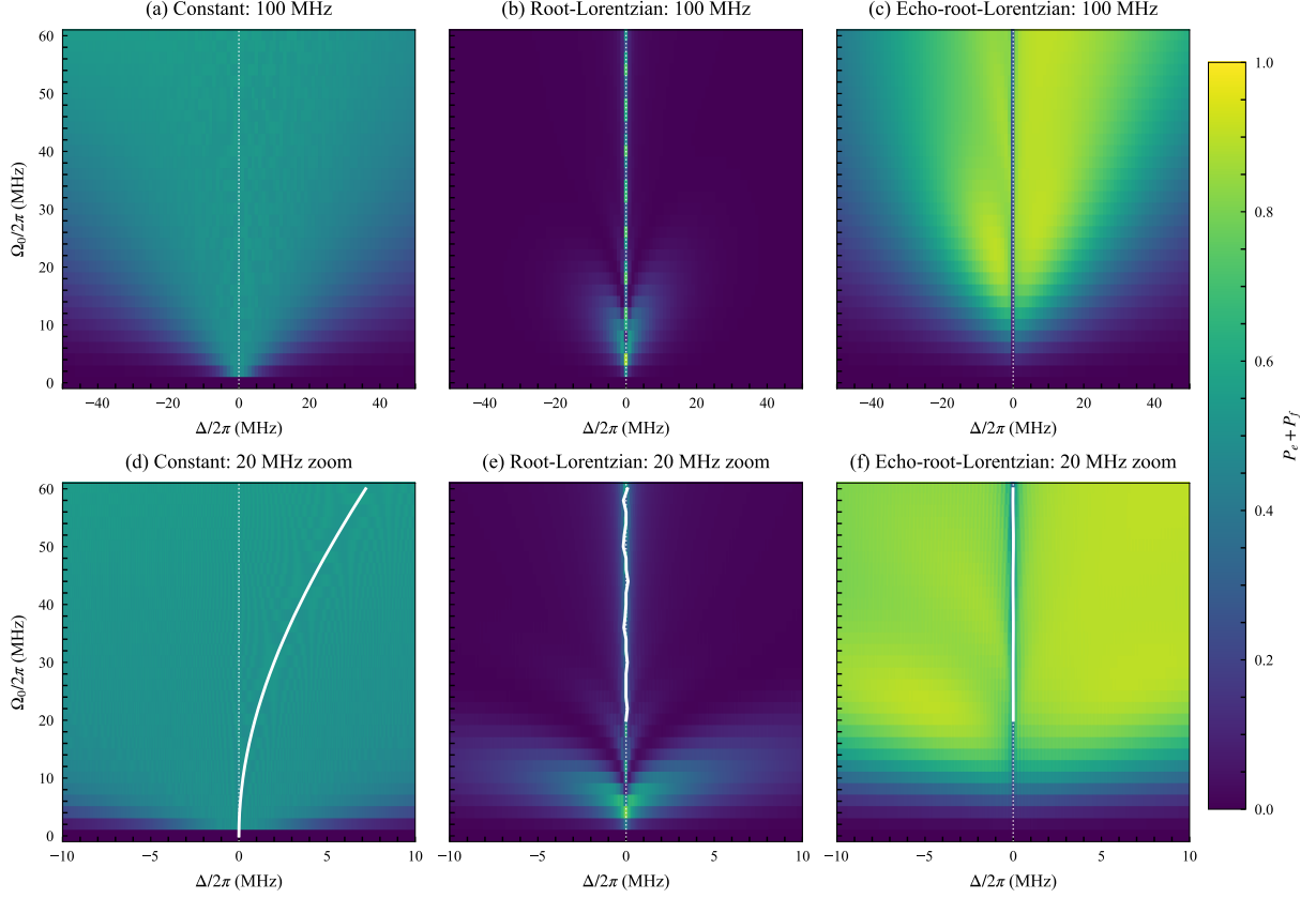
Figure S12. Full-domain and central-zoom three-level calculations of the f_{01} response for a 40 \mu\text{s} constant pulse and 10 \mu\text{s} shaped pulses. (a)–(c) Final excitation P_e + P_f over the full -50 to 50 MHz domain for constant, root-Lorentzian, and echo-root-Lorentzian drives. (d)–(f) Corresponding 20 MHz zooms from -10 to 10 MHz. The dotted line is the bare f_{01} frequency. In the zooms, the solid lines show the exact constant-drive dressed center and the spectral symmetry centers of the root-Lorentzian and echo-root-Lorentzian responses, respectively.
