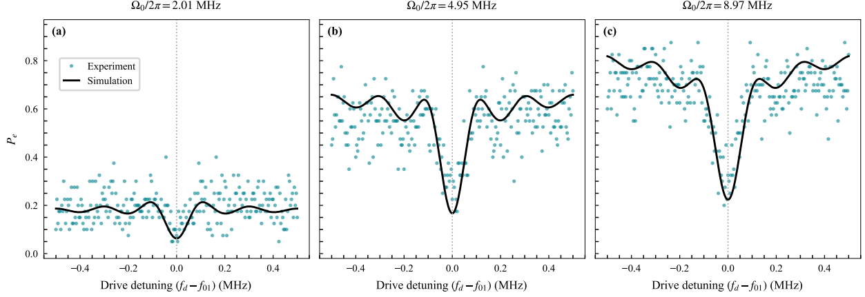
Figure S6. Measured (colored markers) and simulated (black curves) fixed-amplitude spectra at calibrated peak Rabi frequencies \Omega_0/2\pi = 2.011 , 4.951 , and 8.973 MHz. The vertical dotted line denotes zero detuning. For visual clarity, every fourth measured detuning point is displayed; all 1001 points enter the linewidth analysis. The simulation uses the parameters of Fig. S5 without a readout rescaling or fitted frequency shift.
