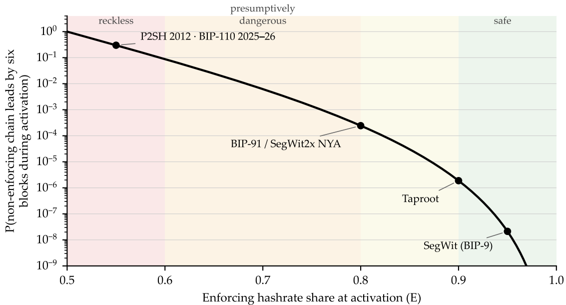
Figure 3.1: Probability that the non-enforcing chain leads the enforcing chain by six blocks at some point during activation, P = ((1 - E) / E)^6 , log scale, as a function of enforcing hashrate share E . Historical thresholds are marked at their signaling values. The curve is a cliff, not a slope.
