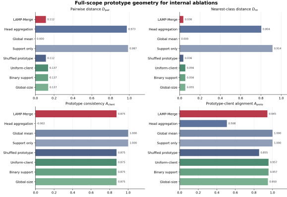
Figure 9: Prototype-geometry comparison on the full benchmark. The figure summarizes pairwise distance, nearest-class distance, prototype consistency, and prototype-client alignment.
