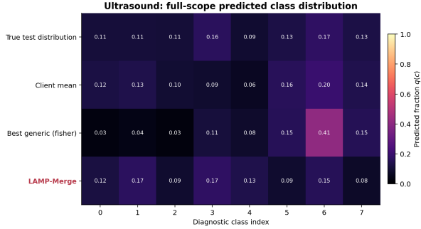
Figure 7: Prediction Distribution on the Ultrasound Dataset
