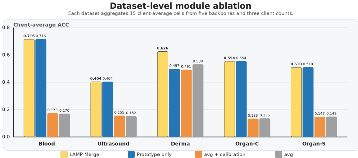
Figure 4: Dataset-level client-average accuracy in the module ablation. Each dataset contains 15 cells from five model families and three client counts; each cell is averaged over three Dirichlet skew levels.
