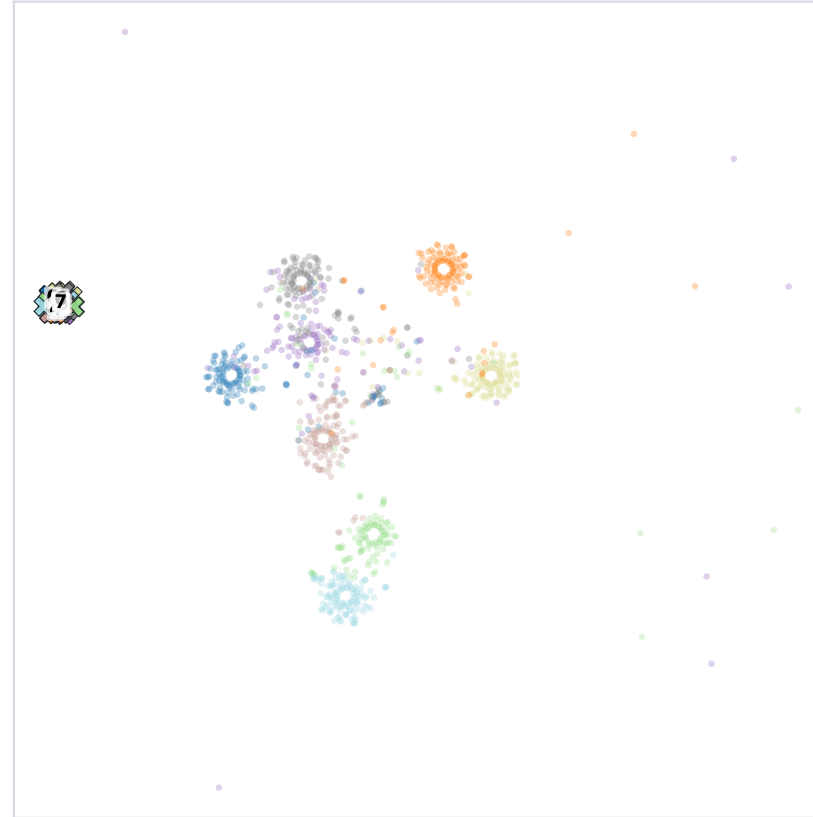
Classifier-head aggregation
