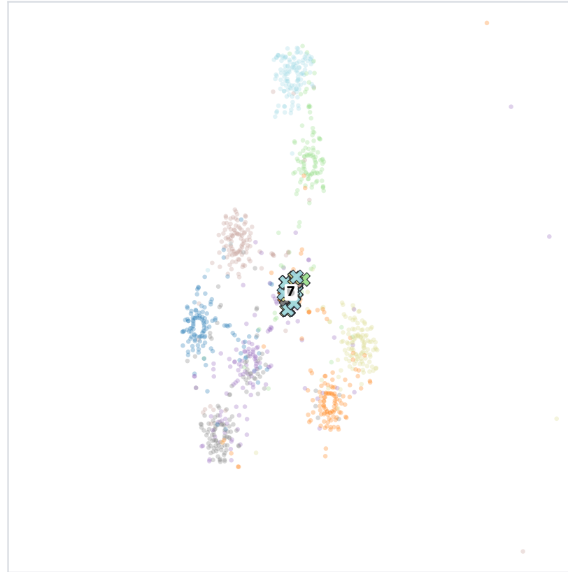
Global-feature mean
