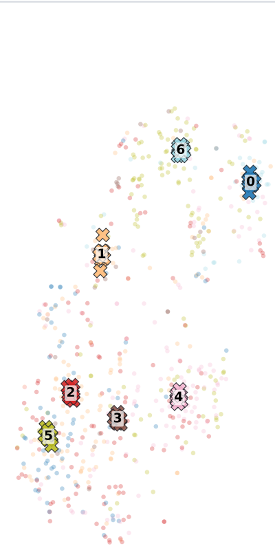
Shuffled-label prototype
