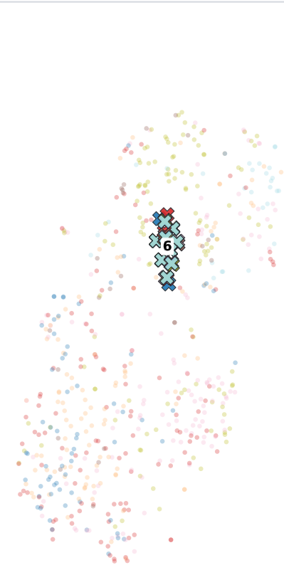
Global-feature mean
