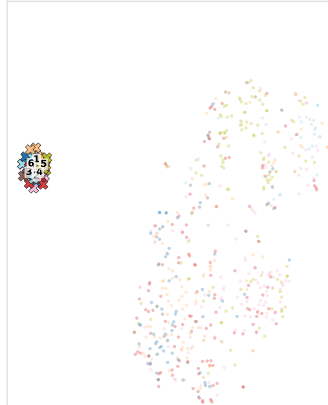
Classifier-head aggregation
