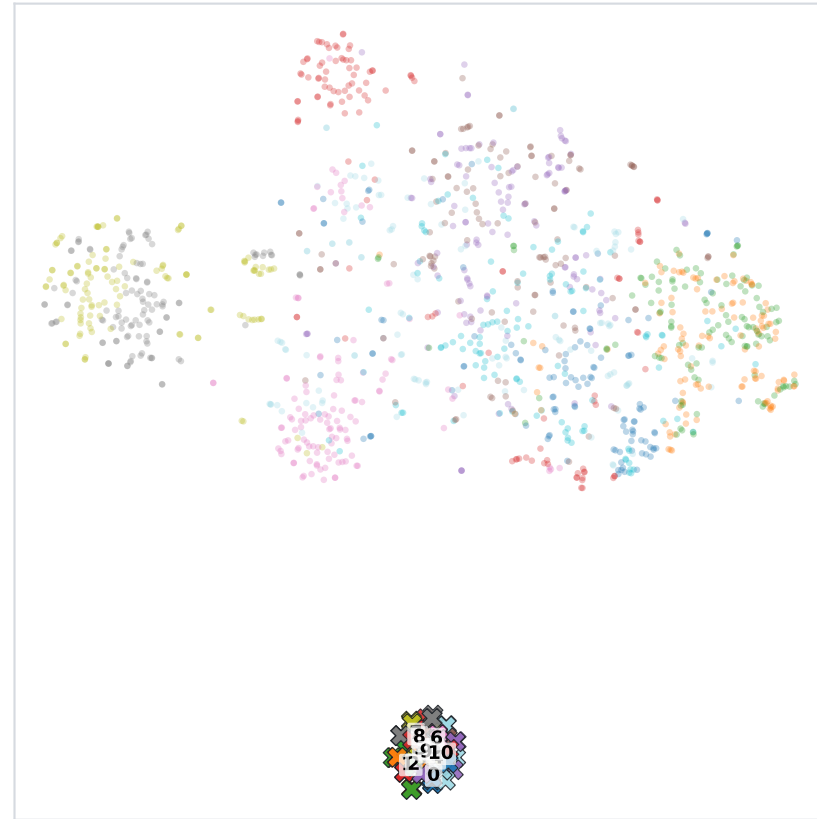
Classifier-head aggregation
