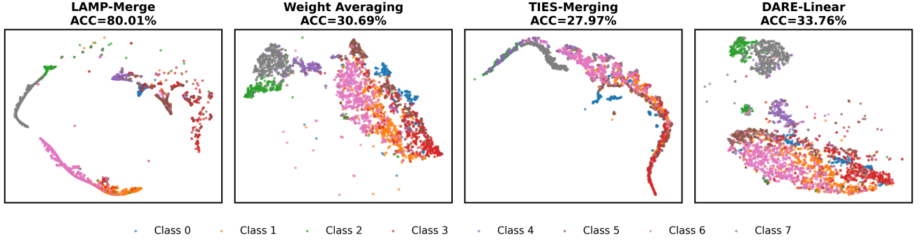
Figure 8: Joint t-SNE of test-image output-probability representations on Blood; from left to right, LAMP-Merge, weight averaging, TIES-Merging, and DARE-Linear.
