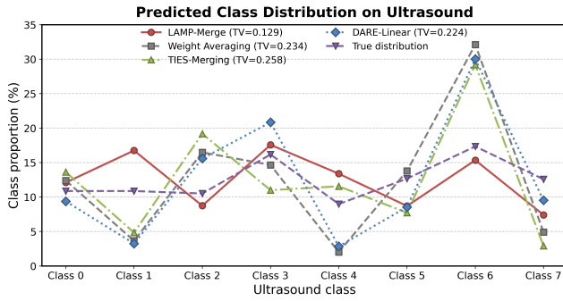
Figure 5: Predicted class distributions on Ultrasound, averaged over the four visual backbones, K \in \{3, 5, 7\} , and the three Dirichlet skew levels. Generic merges concentrate predictions on a few classes, while LAMP-Merge recovers a broader class allocation aligned with the test distribution.
