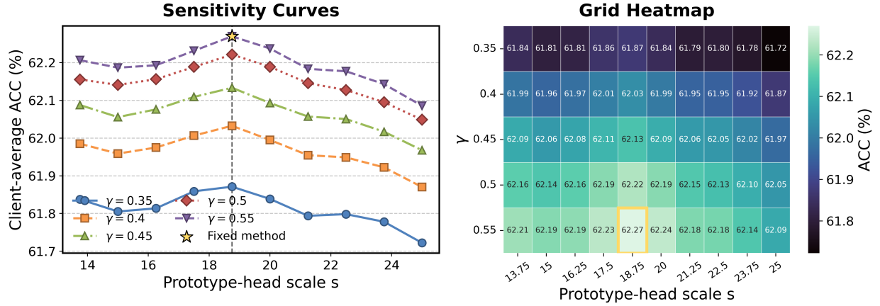
Figure 6: Full-scope hyperparameter sensitivity for diagnostic prototype reconstruction.
