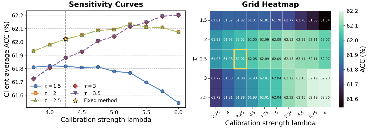
Figure 7: Full-scope hyperparameter sensitivity for long-tail prevalence calibration.
