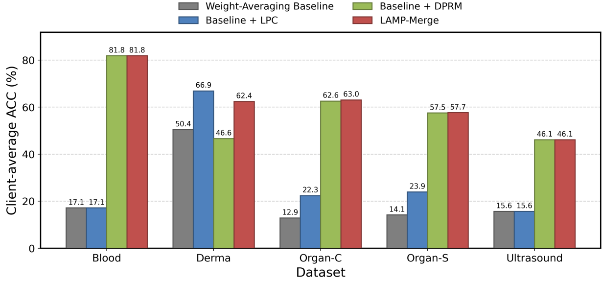
Figure 4: Dataset-level client-average accuracy in the module ablation. Each dataset contains 12 cells from four vision-model families and three client counts; each cell is averaged over three Dirichlet skew levels.
