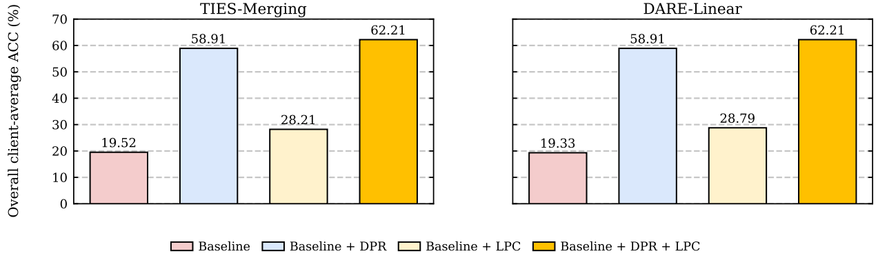
Figure 4: Strict 2 \times 2 DPR/LPC ablations for TIES-Merging and DARE-Linear. Values are overall ACC across 60 client-average cells (five datasets, four backbones, and three client counts).
