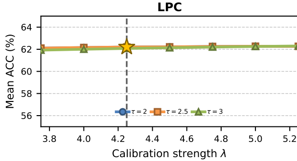
Figure 6: LPC sensitivity under the full LAMP-Merge configuration, with DPR fixed at its selected operating point. Each point averages 60 client-average cells.
