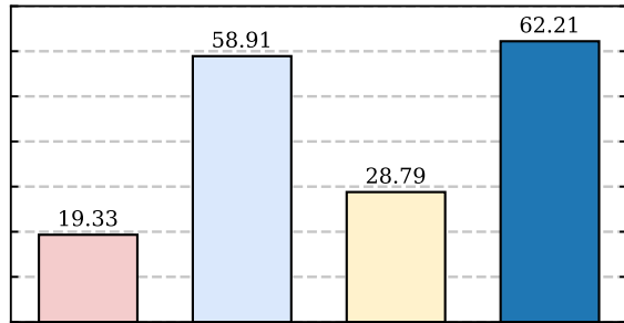
DARE-Linear
