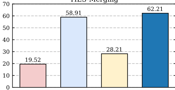
TIES-Merging
