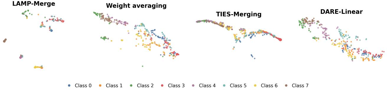
Figure 7: Joint t-SNE visualization of output-probability representations on Blood. From left to right: LAMP-Merge, weight averaging, TIES-Merging, and DARE-Linear.
