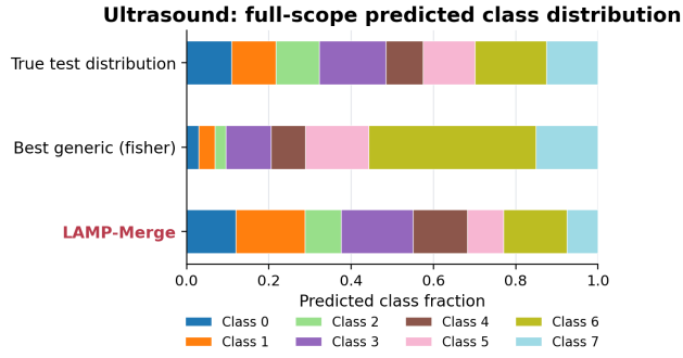
Figure 6: Predicted class distributions on Ultrasound, averaged over the four visual backbones, K \in \{3, 5, 7\} , and the three Dirichlet skew levels. The generic merge concentrates predictions on one class, while LAMP-Merge recovers a broader class allocation aligned with the test distribution.
