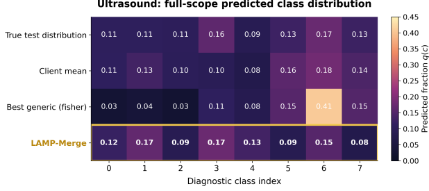
Figure 7: Prediction Distribution on the Ultrasound Dataset
