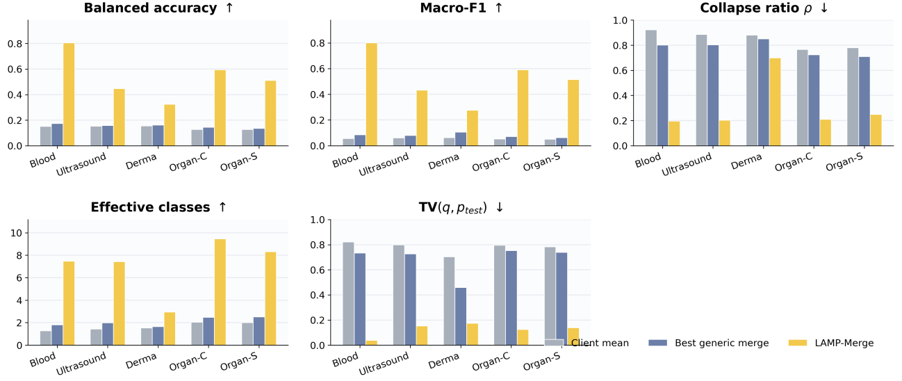
Figure 6: Recovery of global diagnostic discrimination under different datasets.
