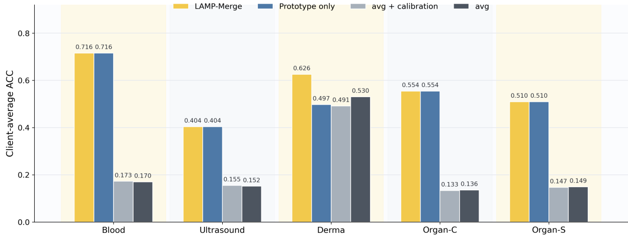
Figure 4: Dataset-level client-average accuracy in the module ablation. Each dataset contains 15 cells from five model families and three client counts; each cell is averaged over three Dirichlet skew levels.
