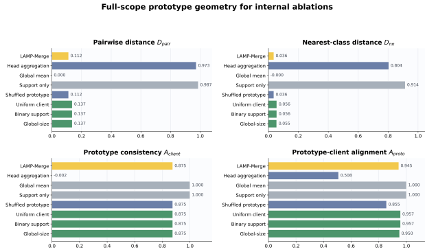
Figure 9: Prototype-geometry comparison on the full benchmark. The figure summarizes pairwise distance, nearest-class distance, prototype consistency, and prototype-client alignment.
