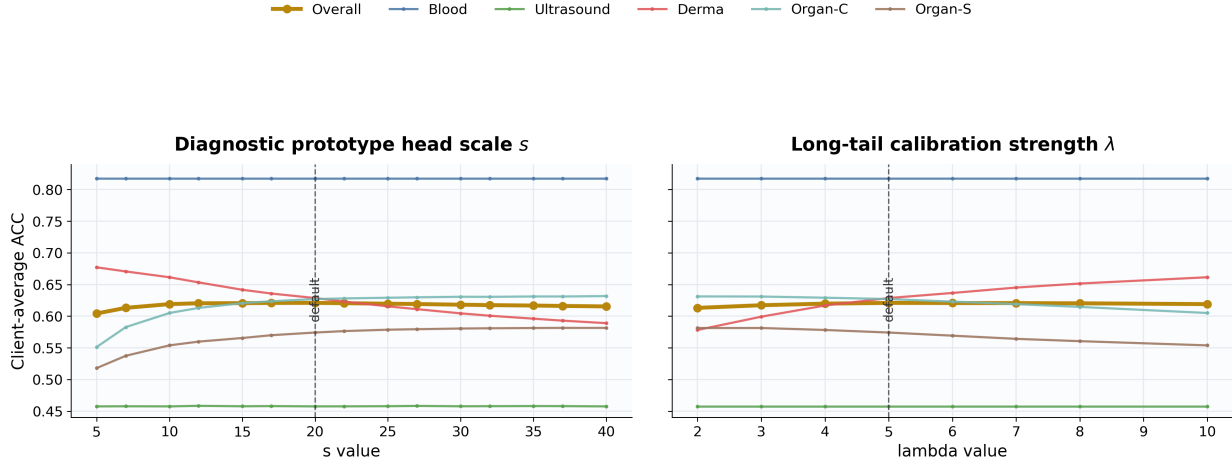
Figure 5: Full-scope hyperparameter sensitivity. The default setting s = 20 and \lambda = 5 lies in the stable high-accuracy plateau.
