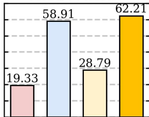
DARE-Linear
