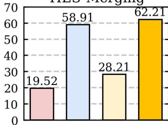
TIES-Merging
