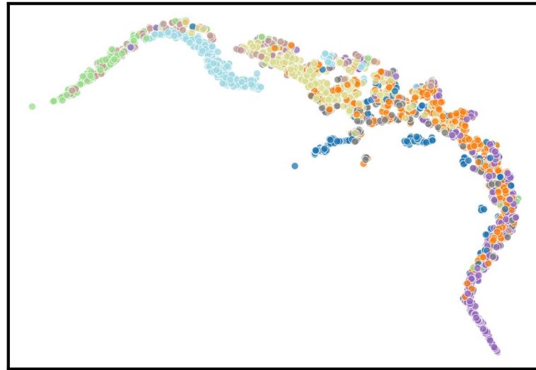
TIES-Merging Acc=27.97%
