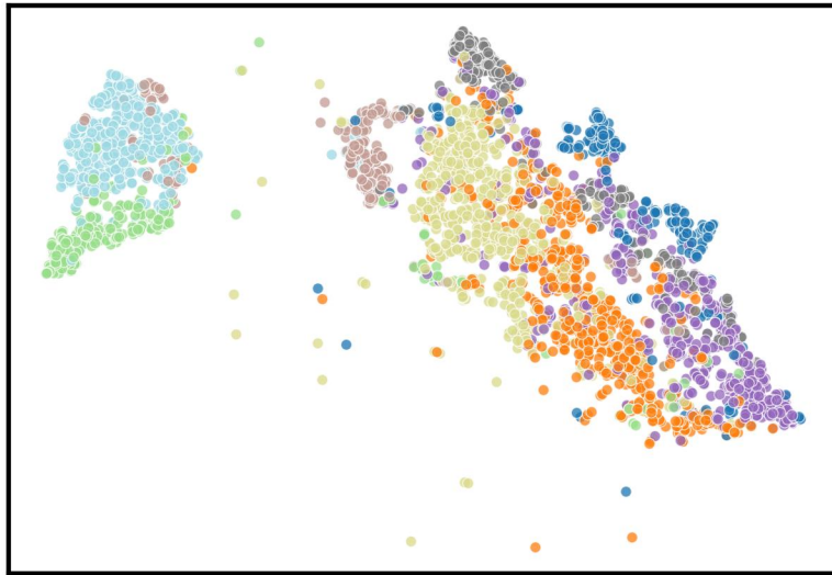
Average Acc=30.69%
