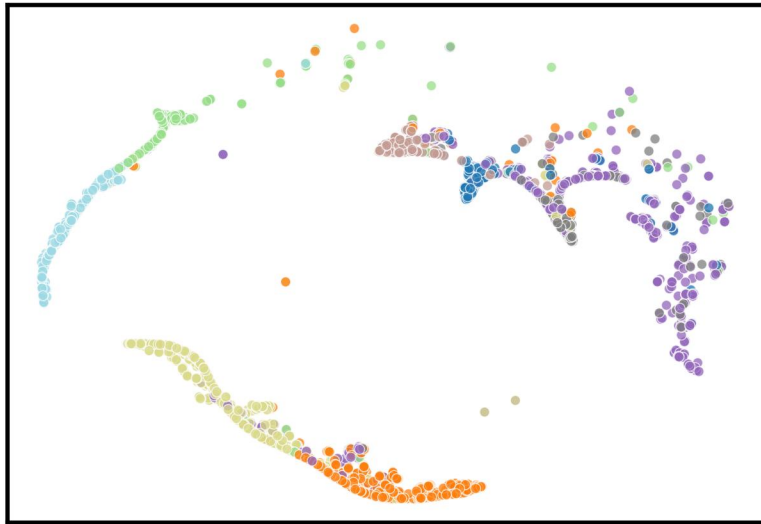
LAMP-Merge Acc=79.95%
