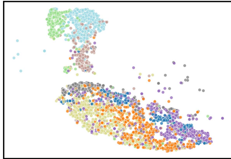
DARE-Linear Acc=33.76%
