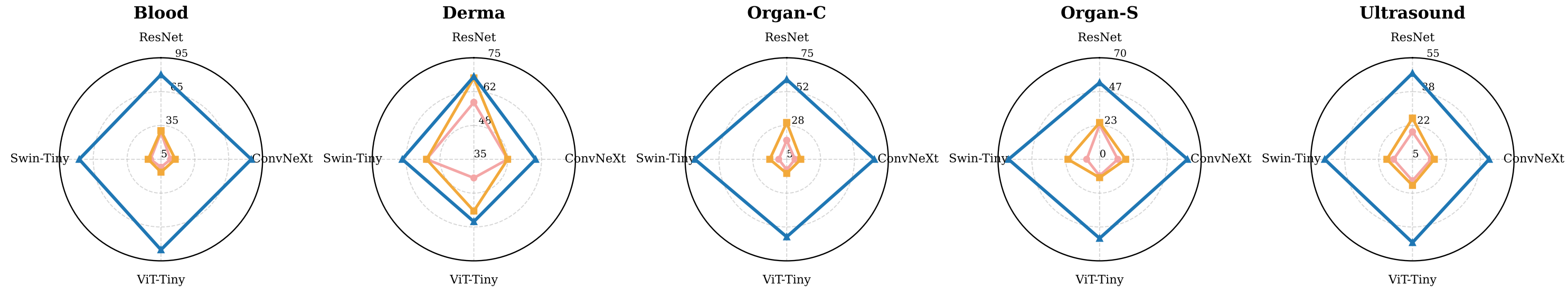
Dataset-level radar comparison over backbone families (client-average ACC).
