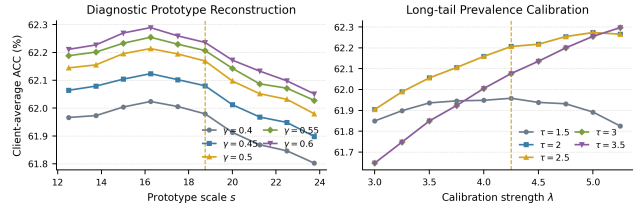
Figure 6: Full-grid DPR/LPC hyperparameter analysis on the full setting ; each curve fixes one module parameter and scans the other over all datasets, backbones, client counts, and Dirichlet settings.
