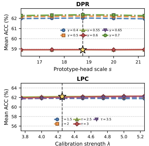
Figure 6: Full-scope DPR and LPC sensitivity. Solid curves use the 2026-07-19 grid; dashed and dash-dotted curves use earlier complete grids. Each point averages 60 client-average cells.
