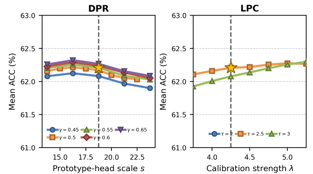
Figure 6: DPR/LPC sensitivity on the full setting.
