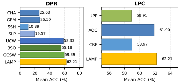
Figure 3: Internal ablations of DPR and LPC. Definitions of the plotted abbreviations are provided in the supplementary ablation configurations.
