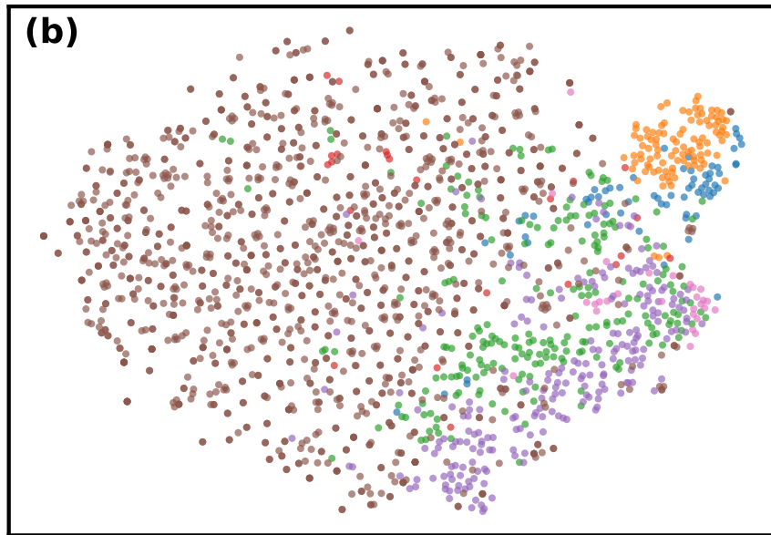
Natural CIFAR ResNet / K=3 / uniform AVG
