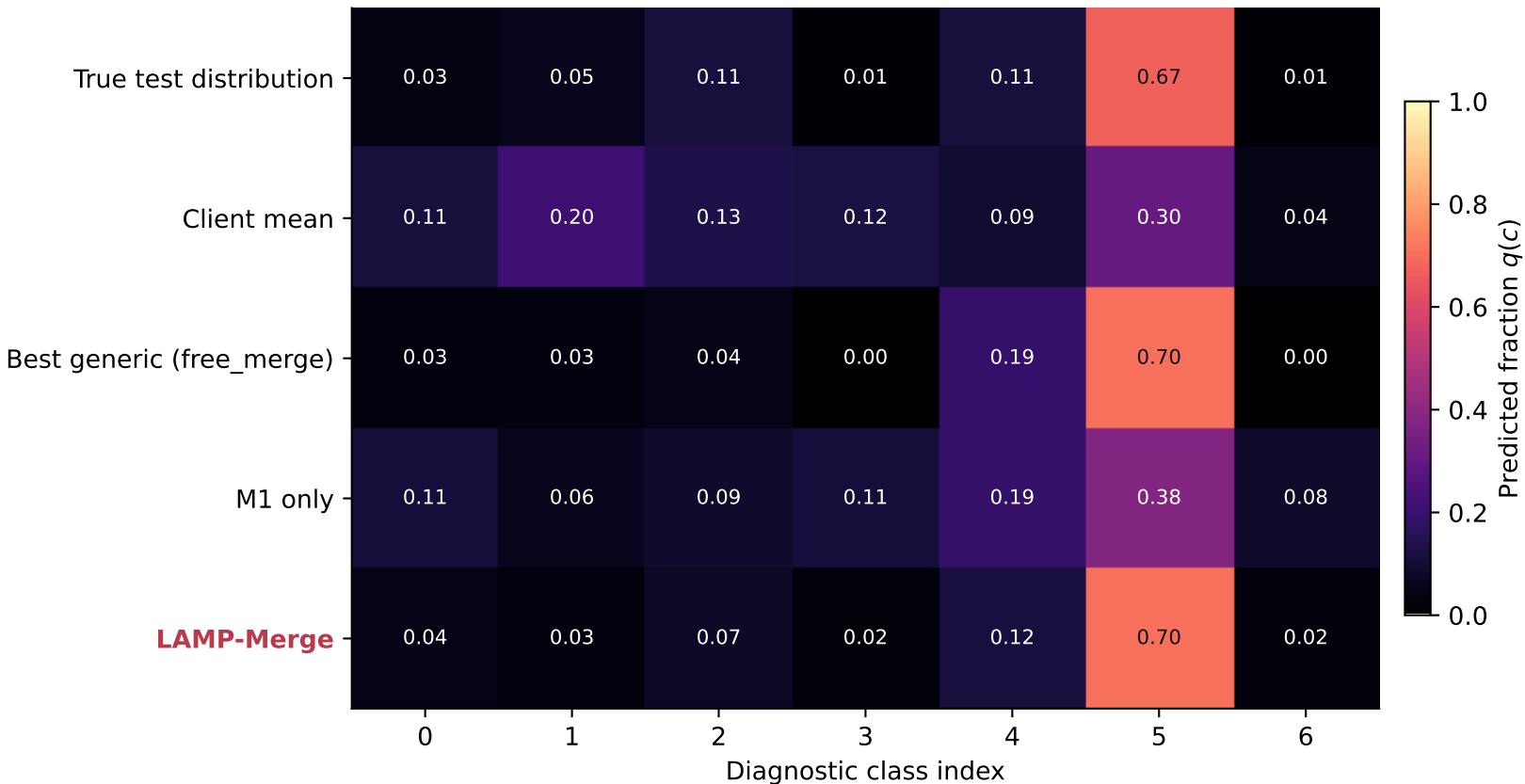
Derma: full-scope predicted class distribution
