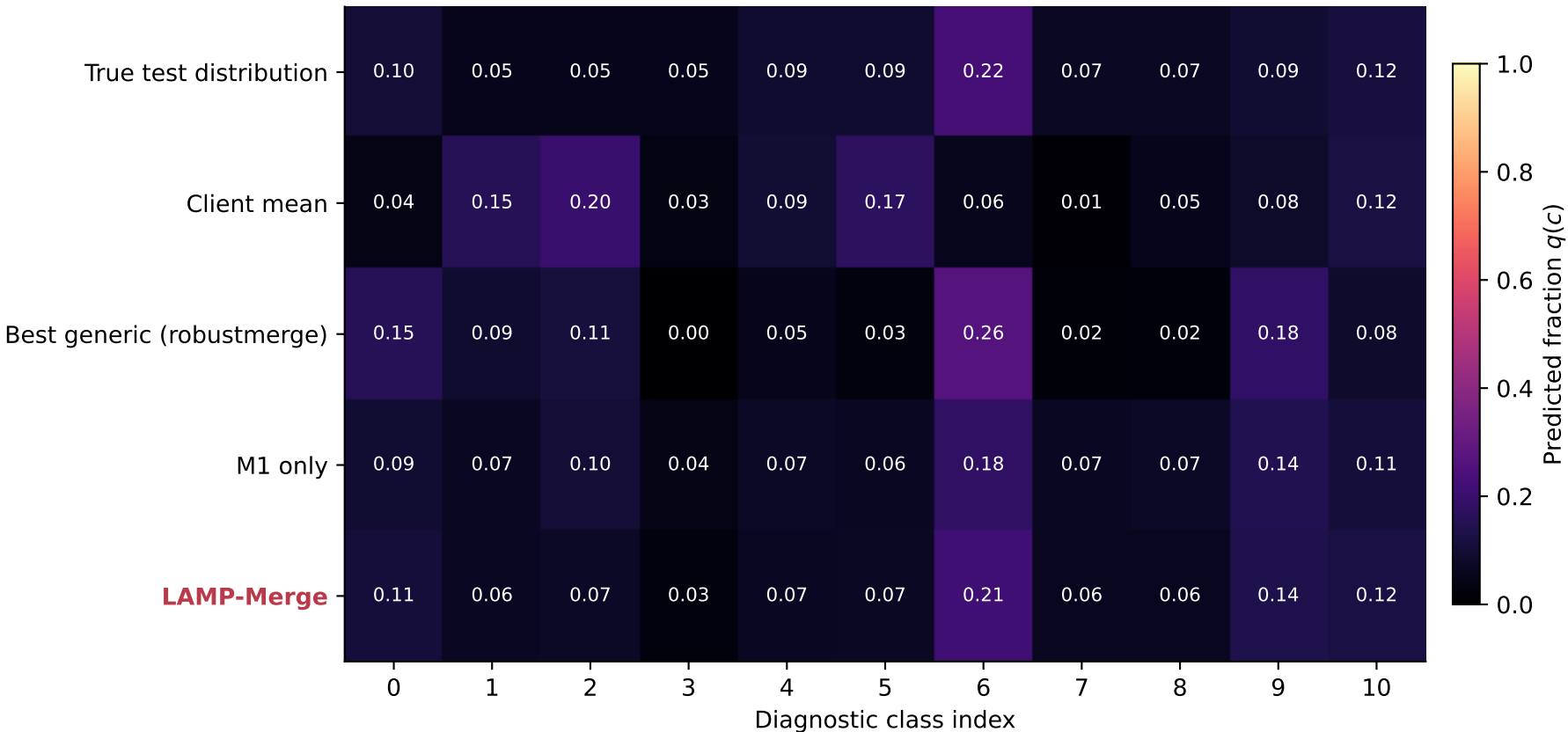
Organ-C: full-scope predicted class distribution
