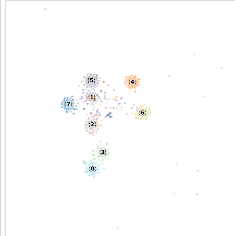
Shuffled-label prototype
