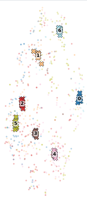
Shuffled-label prototype
