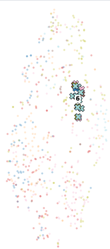
Global-feature mean
