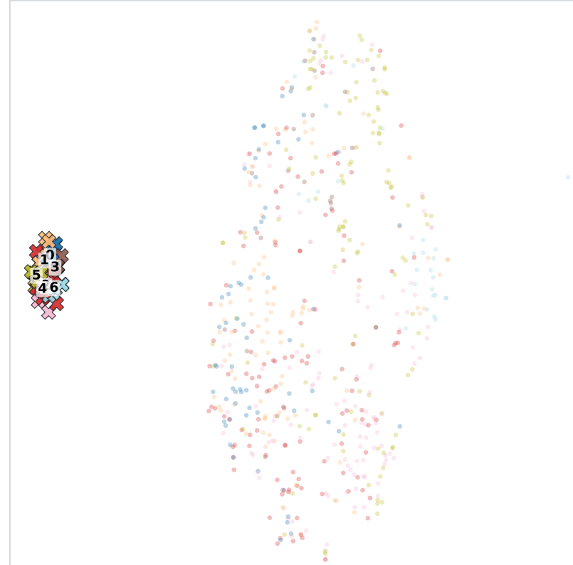
Classifier-head aggregation
